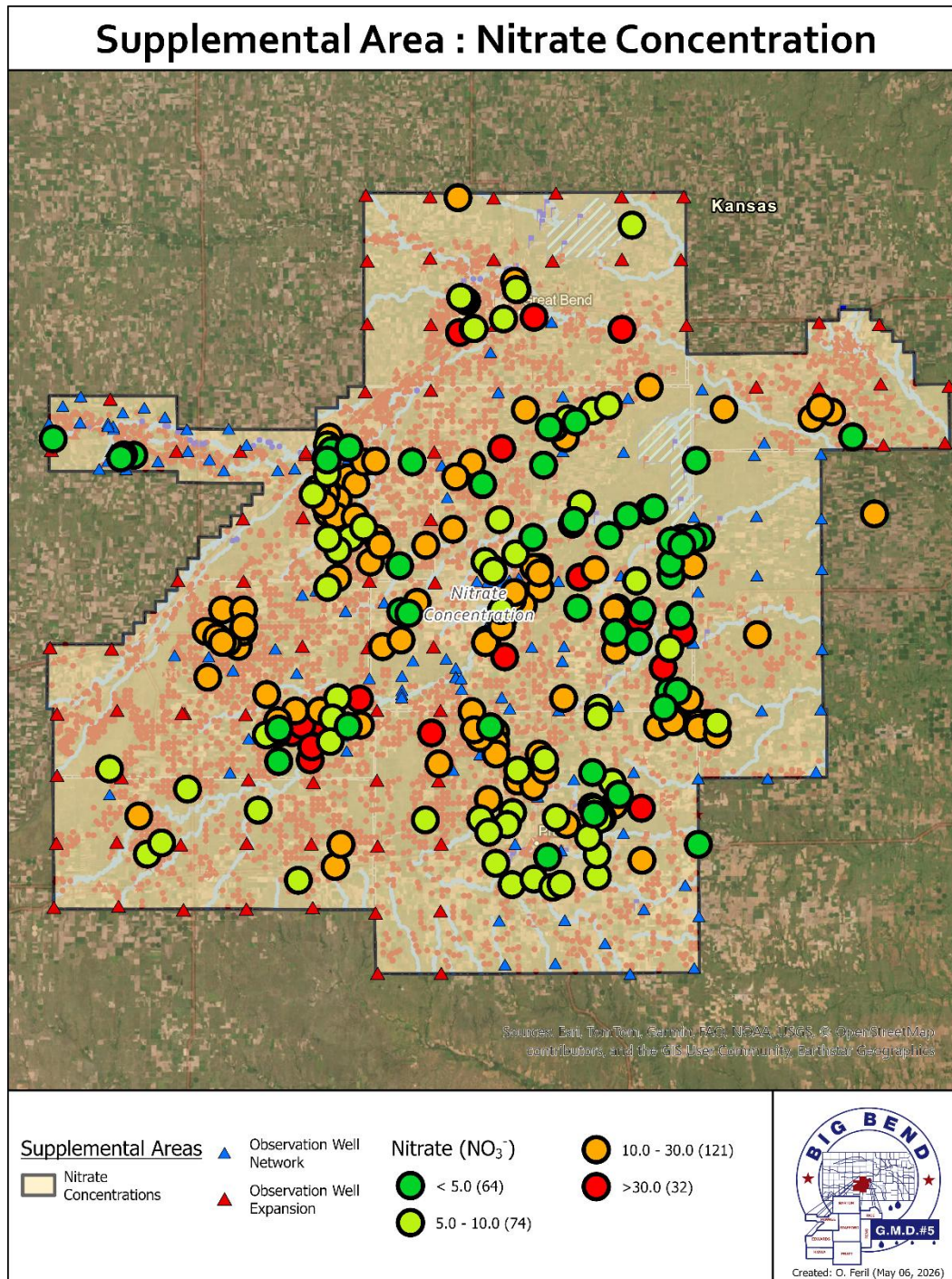
Figure 10 - Nitrate Concentrations
